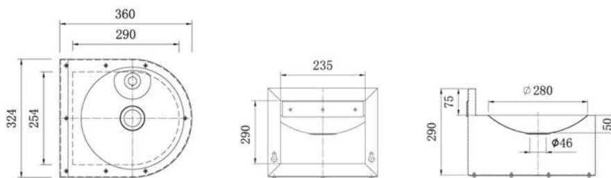
B25 Wall mount drinking fountain with panel
