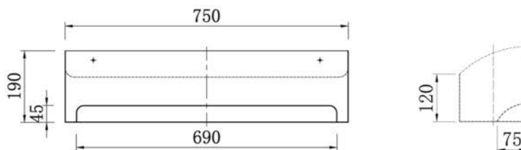
DEV-1043(C75X17X19) Inner tray
