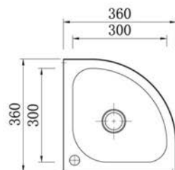
T04-1 Corner sink
