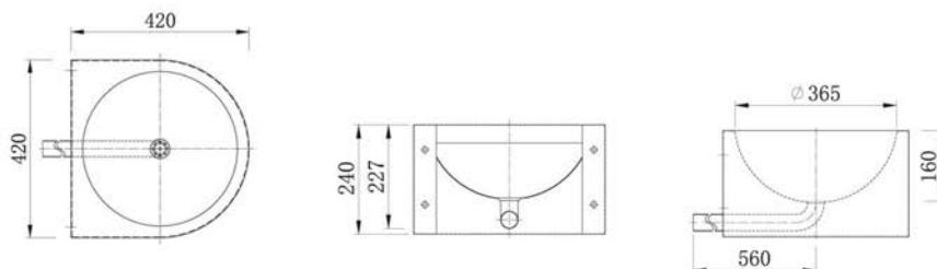
B04-10 Wall mount drinking fountain
