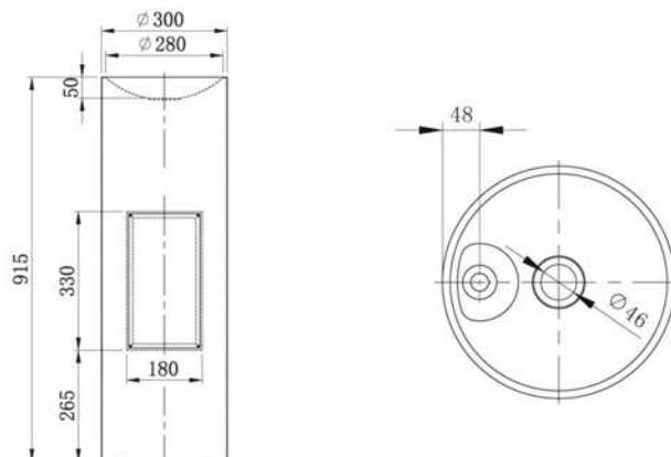
DR-300 Drinking fountain round
