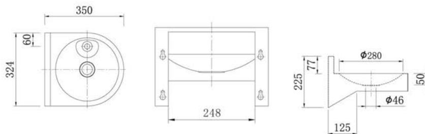
B25-1 Wall mount drinking fountain with panel
