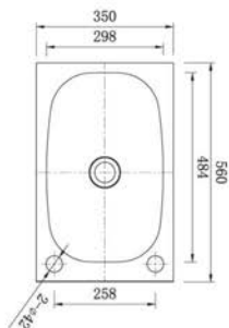
30L Laundry sink & Cabinet
