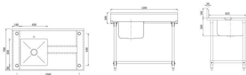
Compartment sink
