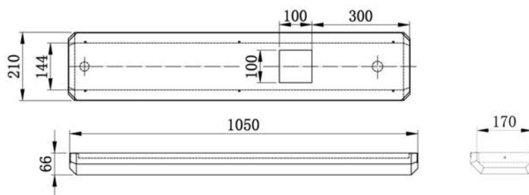
Shower panel
